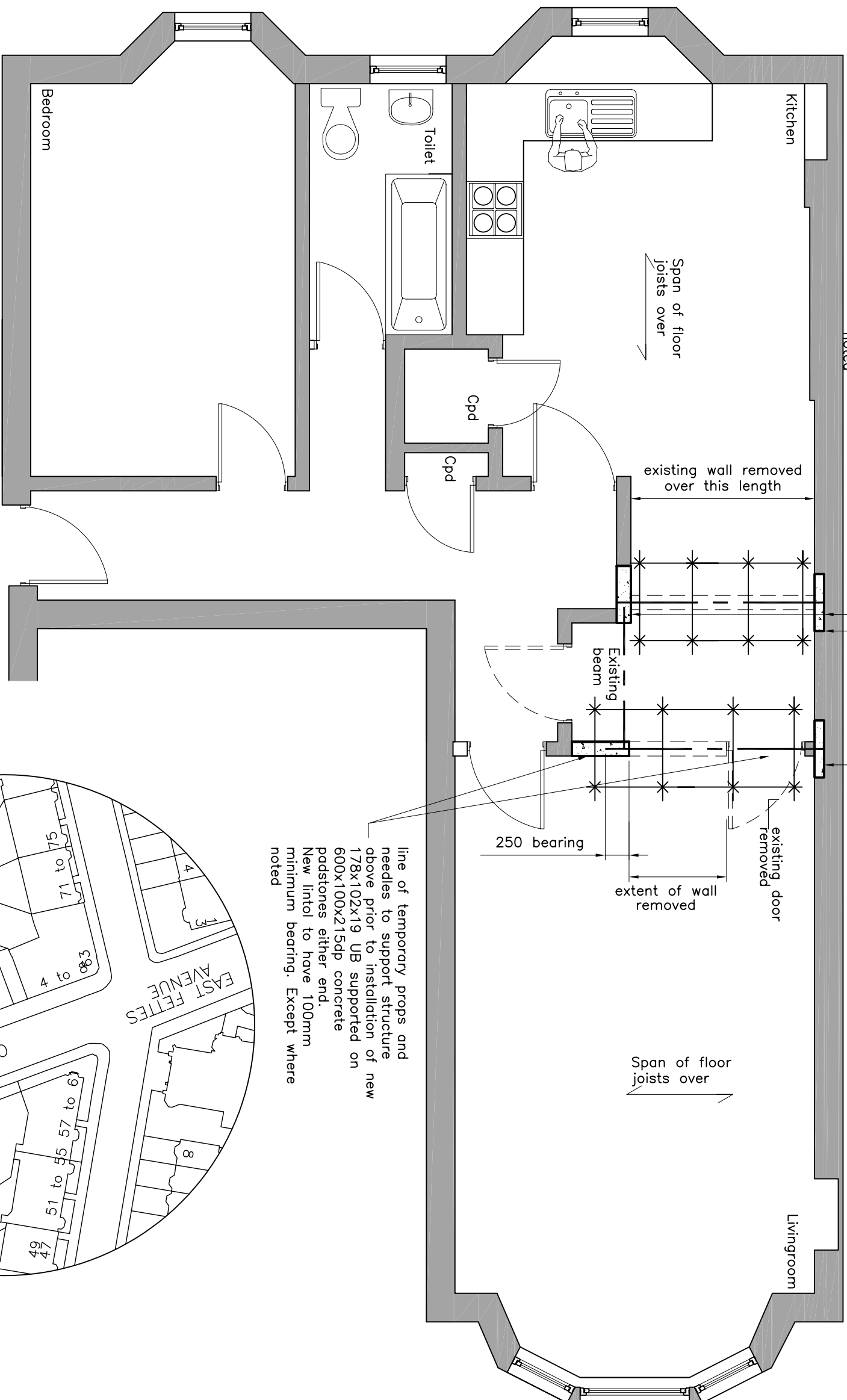
Existing Floor Plan 1:50
